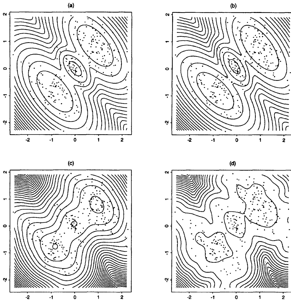
Figure 10. Comparative Density Estimates for Trimodal Multivariate Normal Data. (a) Density used to generate the data; (b) density estimate via model-based clustering; (c) Gaussian kernel density estimate with normal optimal bandwidth; (d) Gaussian kernel density estimate with cross-validated bandwidth. There are 250 data points, superimposed on the contours to show their location.
