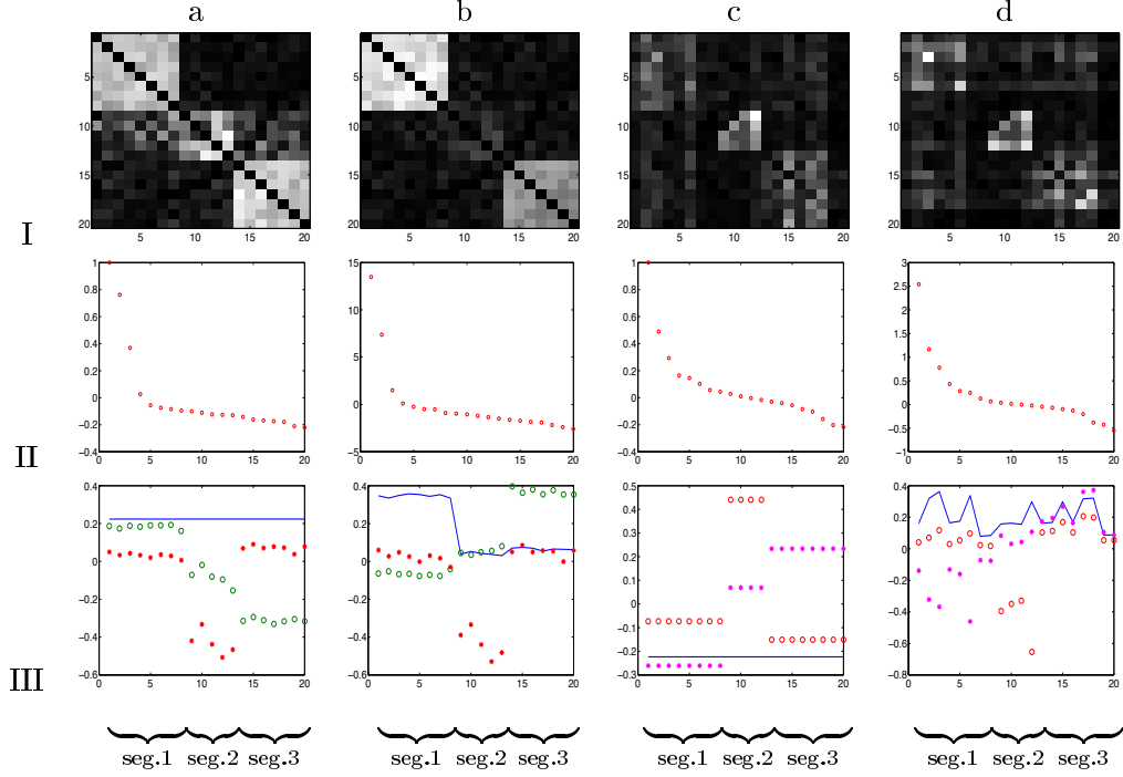
Figure 1: Four matrices (row I), their eigenvalues (row II) and first 3 eigenvectors: x^1 ‘—’, x^2(=x^L in b,d) ‘o’, x^3 ‘*’ (row III). All matrices are represented on a gray-scale with black for 0 and lighter shades for higher values. All matrices correspond to “images” of 20 pixels forming 3 segments. (a) An approximately block-diagonal stochastic matrix P_1 . The second and third eigenvector are approximately piecewise constant and contain information about the segmentation. (b) The symmetric similarity matrix which produced P_1 . Note that all three first eigenvectors contain information about the segmentation. The eigenvectors solving (2) for this matrix are identical to the eigenvectors of P_1 . (c) A block-stochastic matrix P_2 . The second and third eigenvectors are piecewise constant and reflect the correct segmentation. (d) The symmetric similarity matrix that produced P_2 . The first 3 eigenvectors are only roughly piecewise constant and result in a wrong segmentation.
