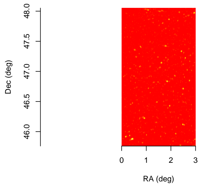
Thresholded Test Statistics
