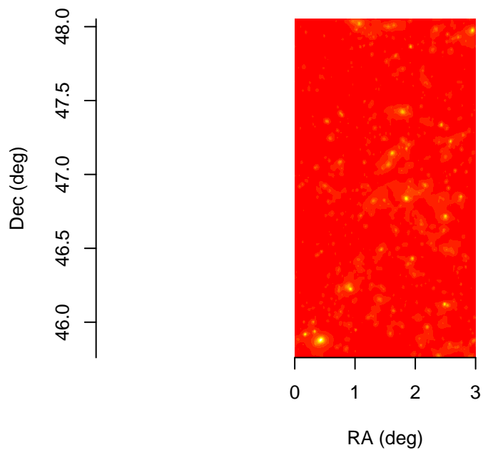
Noise Free Image, blurred
