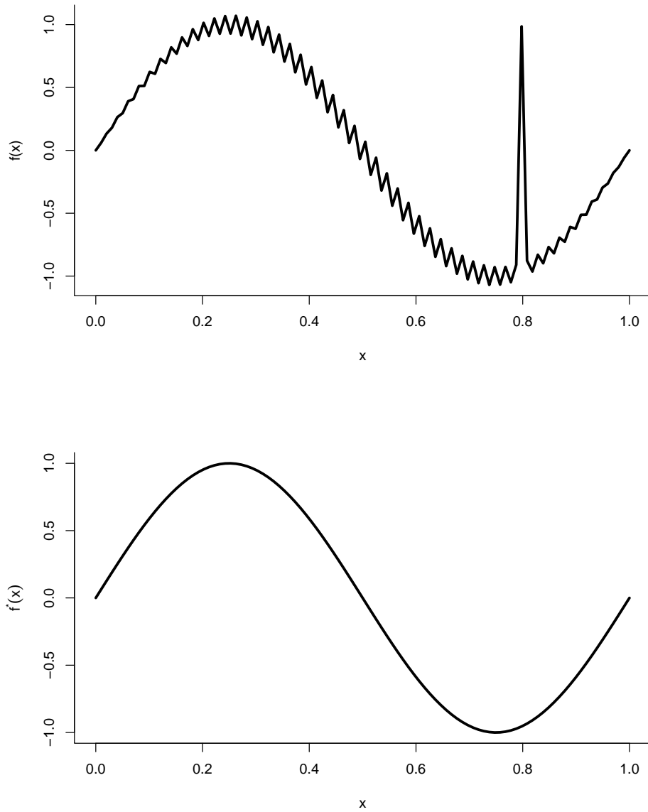
FIG 2. The top plot shows a complicated function f . The bottom shows a surrogate f^* which is simpler than f but retains the main, estimable features of f . Adaptation is possible if we cover f^* instead of f .
