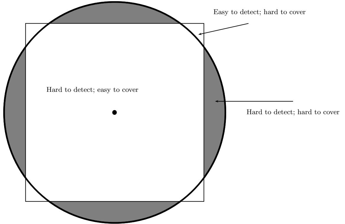
FIG 3. The dot at the center represents the subspace \mathcal{F} . The shaded area is the set of spoilers \mathcal{S}(\epsilon_2, \epsilon_\infty) of vectors for which f^* \neq f . If these vectors were not surrogated, adaptation is not possible. The non-shaded area is the invariant set \mathcal{I}(\epsilon_2, \epsilon_\infty) = \{f : f^* = f\} .
