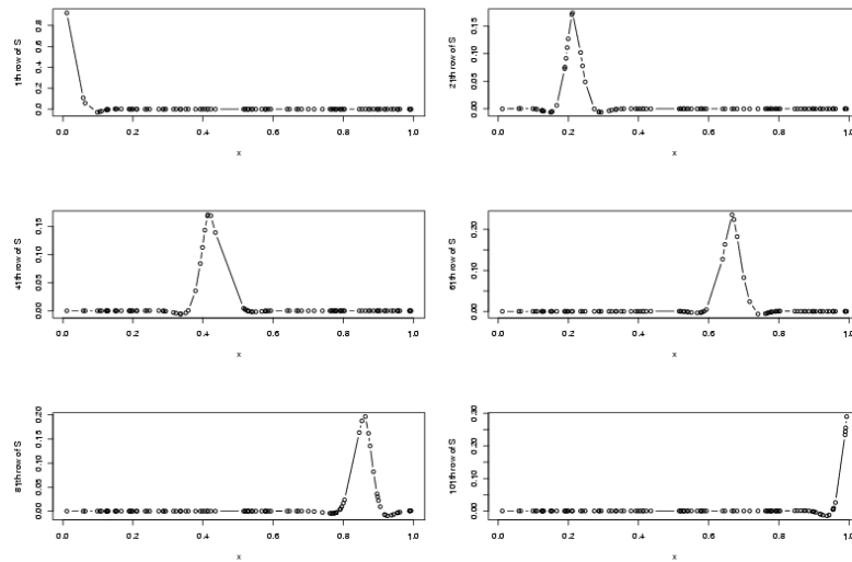
Figure 9.7: Kernels of a smoothing spline.
