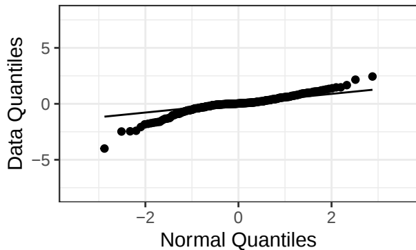
Standardized eta1
