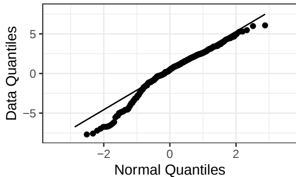
Standardized eta0
