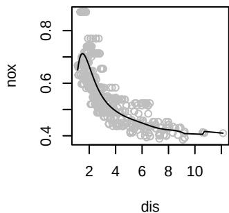
Polynomial of degree 10 RSS = 1.83
