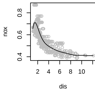
Polynomial of degree 9 RSS = 1.83
