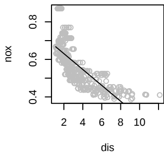
Polynomial of degree 1 RSS = 2.77
