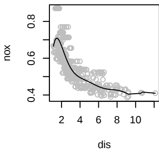
Polynomial of degree 8 RSS = 1.84
