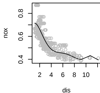
Polynomial of degree 6 RSS = 1.88
