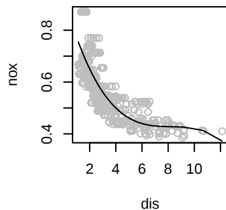
Polynomial of degree 3 RSS = 1.93
