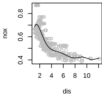
Polynomial of degree 7 RSS = 1.85
