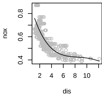
Polynomial of degree 4 RSS = 1.93
