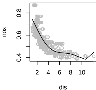
Polynomial of degree 5 RSS = 1.92
