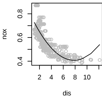
Polynomial of degree 2 RSS = 2.04
