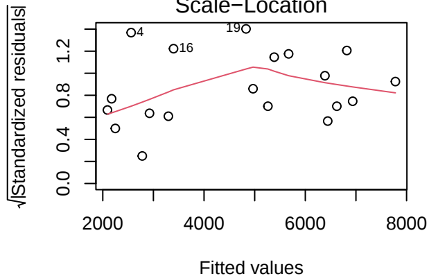
Scale-Location
