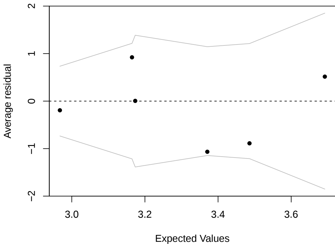
Binned residual plot
