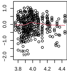
Residuals vs Fitted
