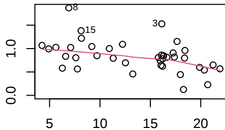
Scale-Location
