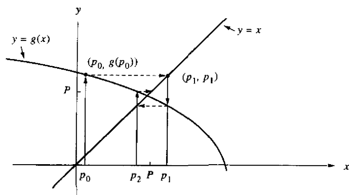
Figure 2.4 (b) Oscillating convergence when -1 < g'(P) < 0 .
