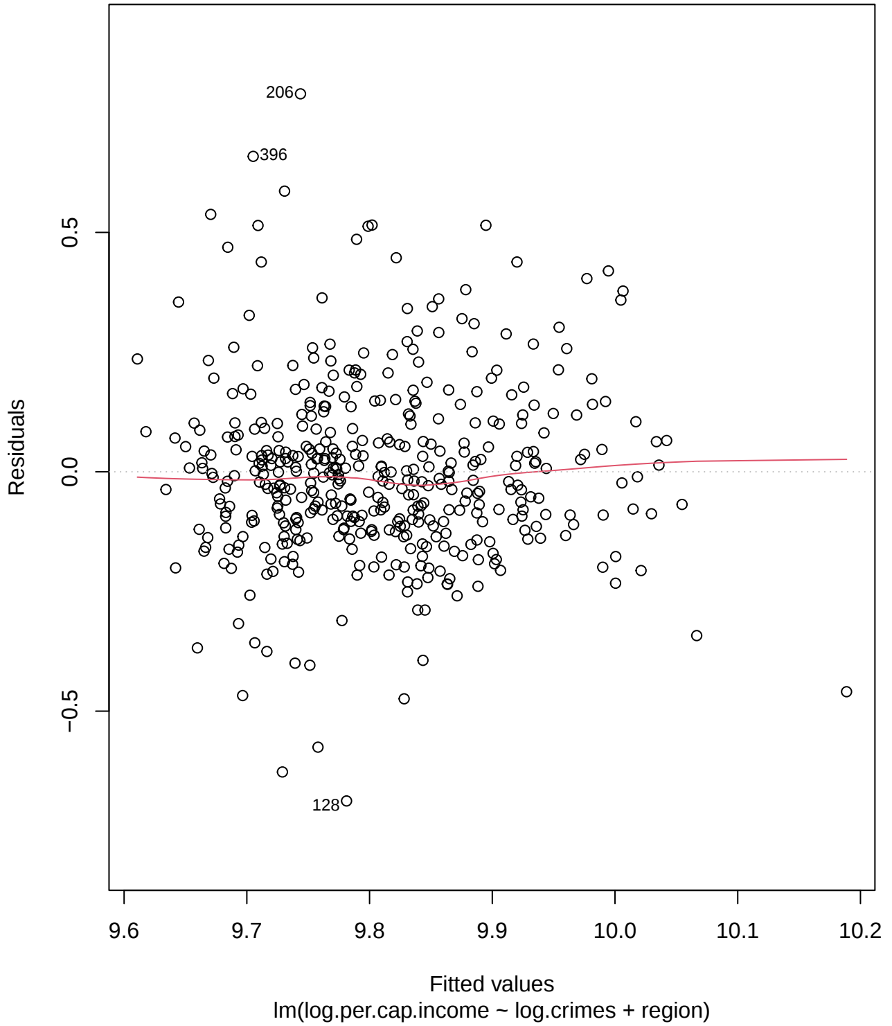
Residuals vs Fitted
