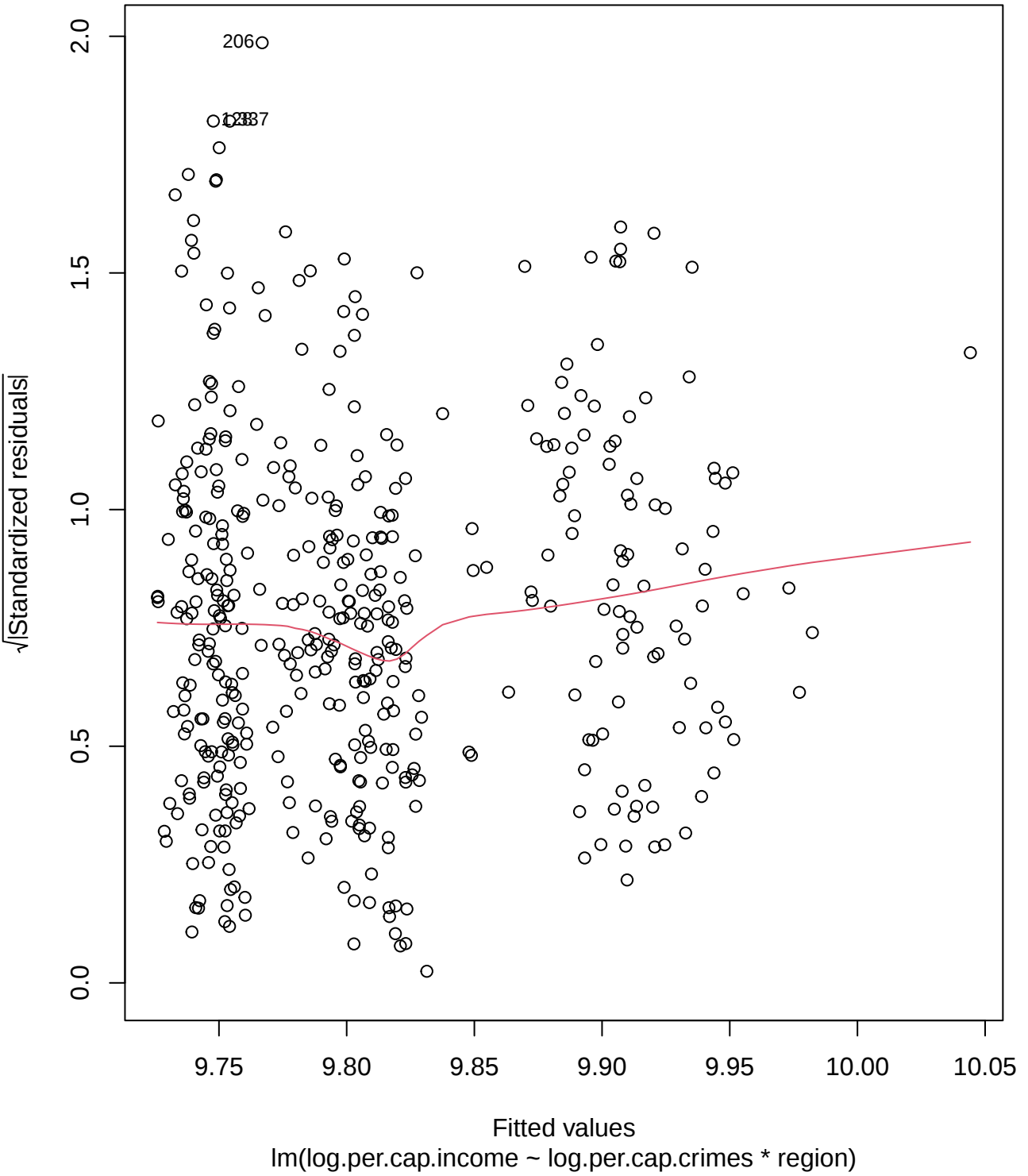
Scale-Location
