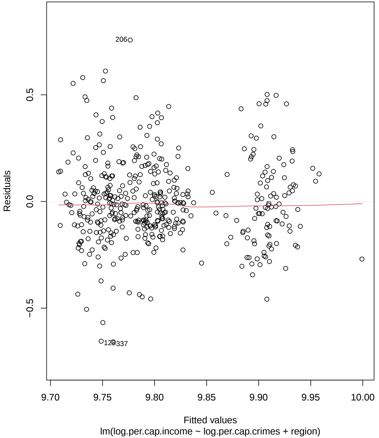
Residuals vs Fitted
