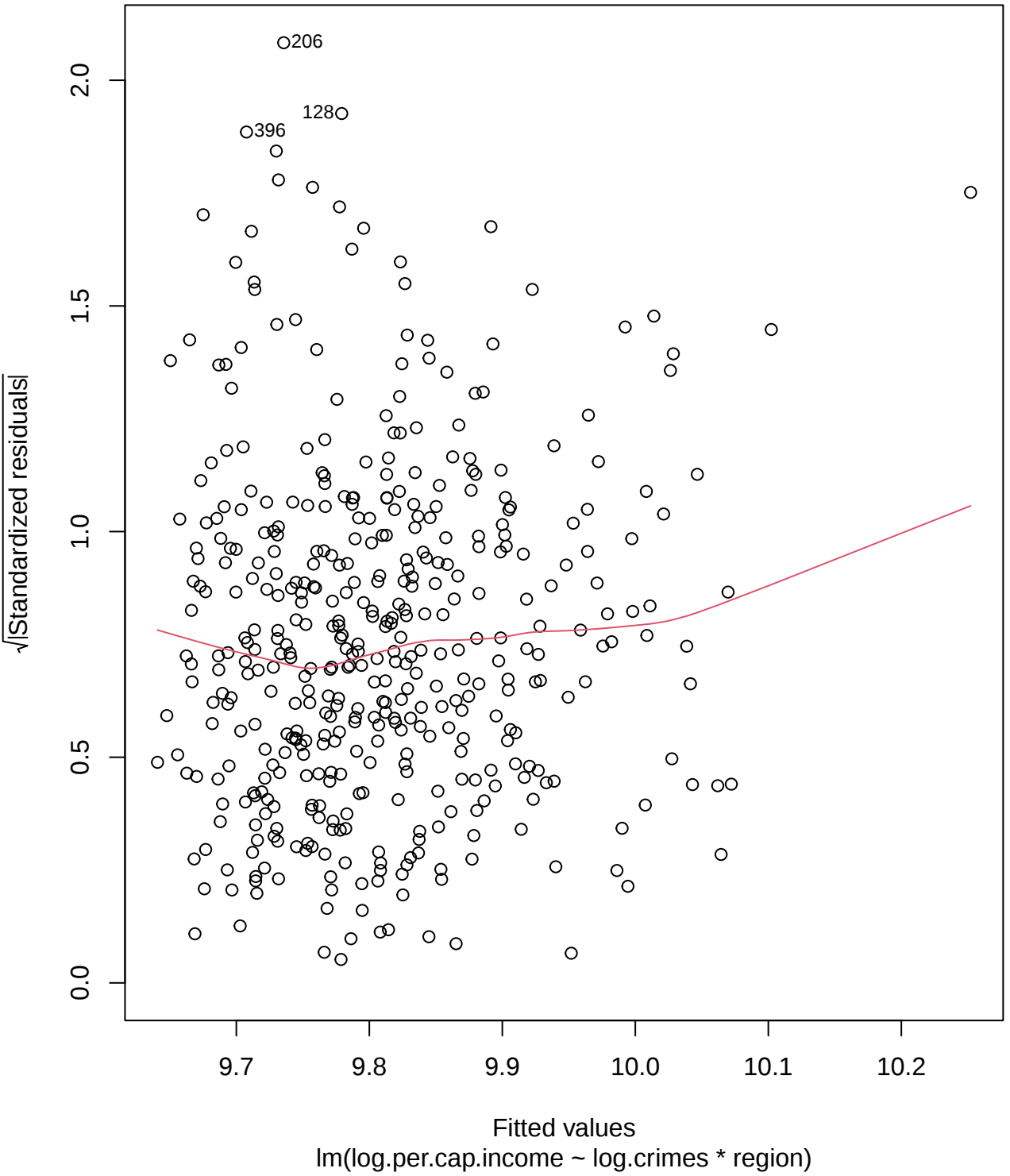
Scale-Location
