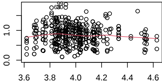
Scale-Location
