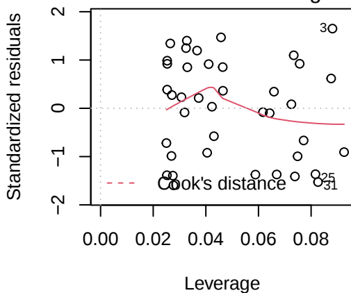
Residuals vs Leverage
