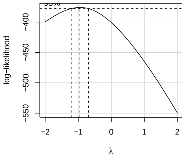
Profile Log-likelihood
