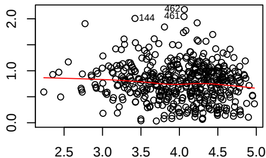
Scale-Location
