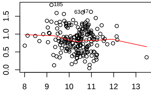
Scale-Location
