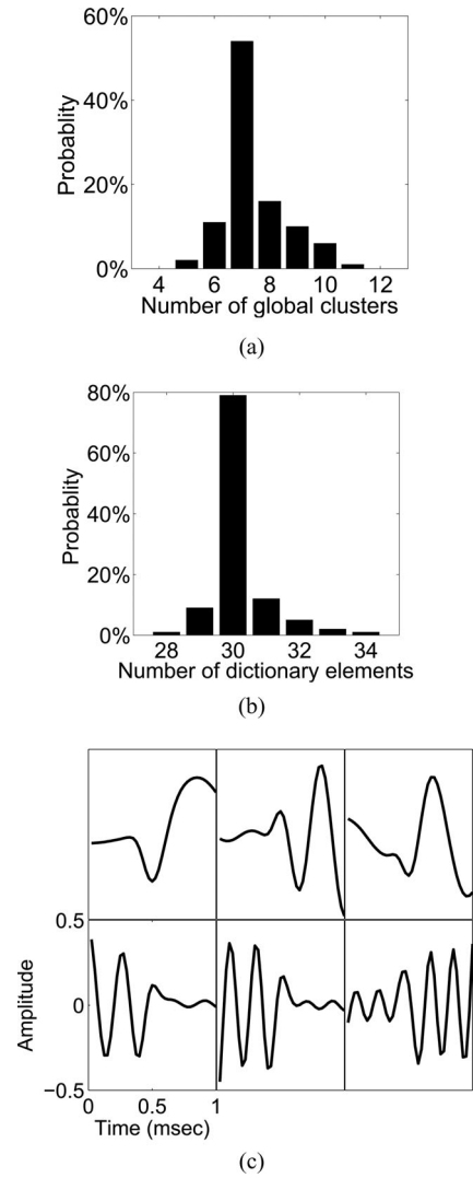
Fig. 4. Posteriors and dictionaries from rat motor cortex data (the same data as in Fig. 3). (a) Approximate posterior distribution on the number of global clusters (mixture components). (b) Approximate posterior distribution of the number of dictionary elements. (c) Examples of inferred dictionary elements; amplitudes of dictionary elements are unit less.
