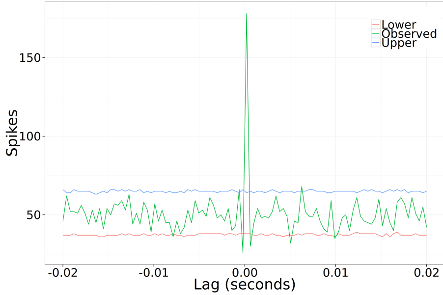
Figure 6: Crosscorrelogram: the lower and upper intervals indicate a 95% bootstrap interval
