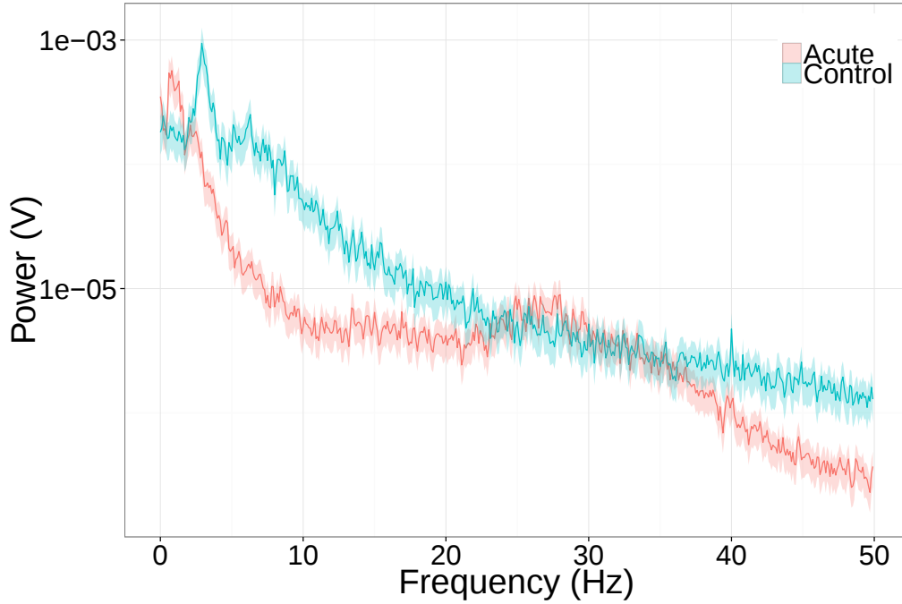
Figure 2: We can see the increased \beta -oscillations as a bump in the power spectrum of the LFP signals.
