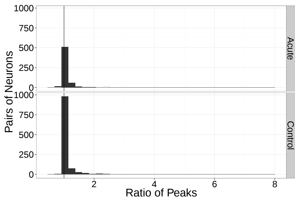
Figure 7: Ratio between observed and bootstrap peaks
