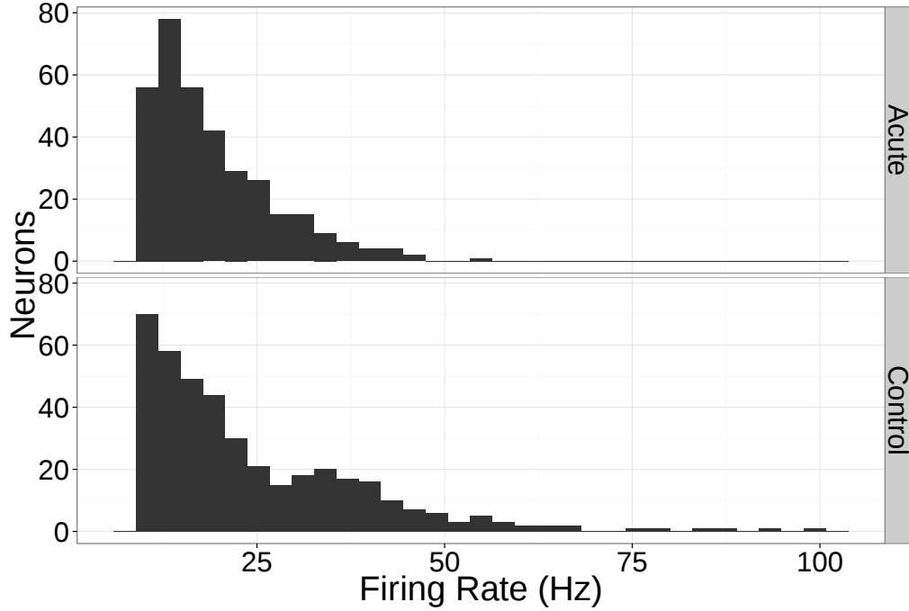
Figure 4: Firing rates for all detected and sorted neurons by condition
