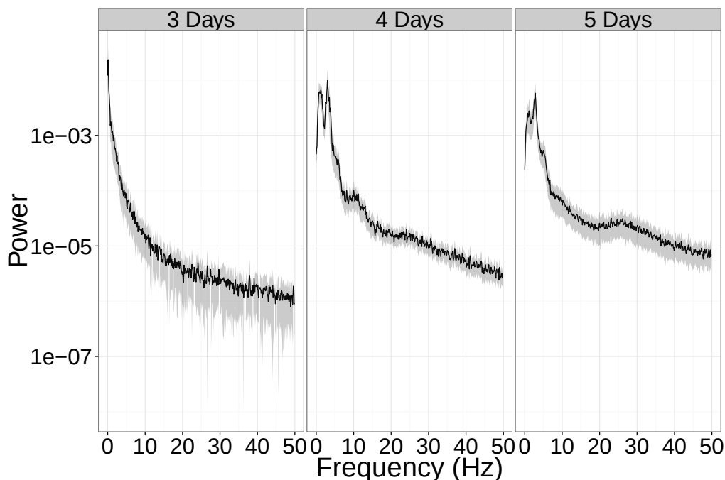
Figure 3: We can see the average spectrum recorded at 3, 4, and 5 post-depletion. We see a bump in the LFP signal develop.
