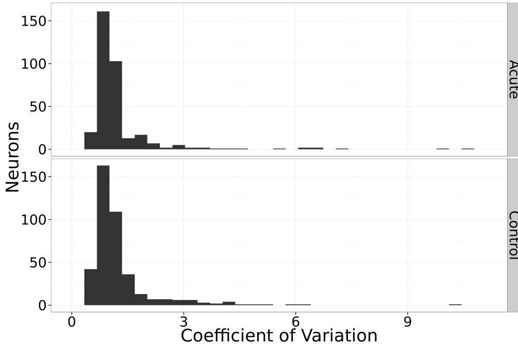
Figure 5: We see little difference in ISI CVs between Acute and Control mice.
