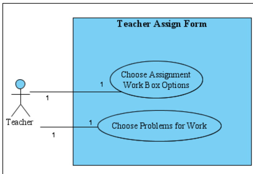
Figure 8.2.4. Use Case diagram for PeerASSIST functionality at the assign page.
