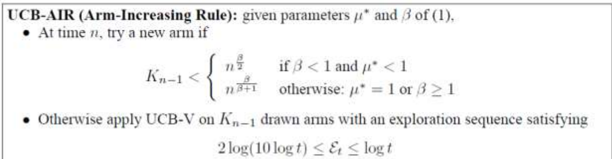
Figure 8.3.4.1: UCB-AIR Allocation Strategy ( Wang et al., 2009 )
