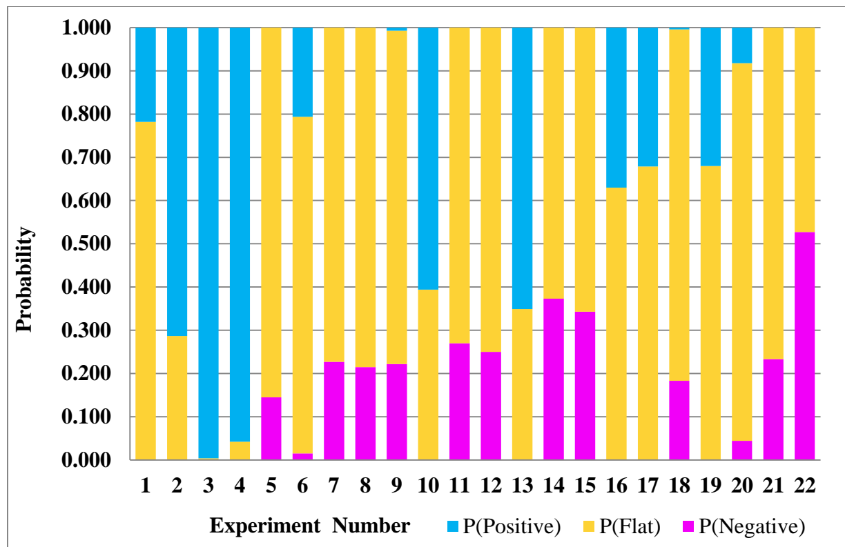
Figure 7.3. A stacked bar graph to show the three probabilities (positive, negative, flat/null) for each experiment.
