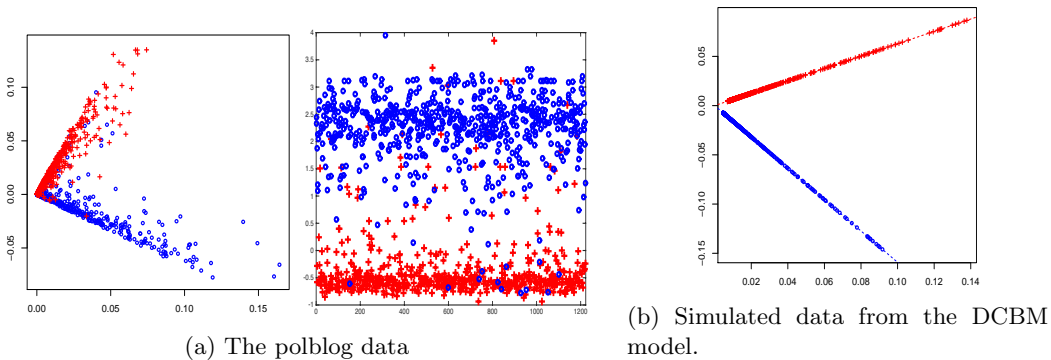
Figure 1: In (a), we plot the rows of \widehat{\Xi} (left) and \widehat{R} (right) for the Polblogs network. In (b), we plot the rows of \Xi using a network simulated from models (1.2)-(1.3) ( n = 1222 , (a, b, c) = (1, 0.1, 1) and \theta_1^{-1}, \dots, \theta_n^{-1} are iid from \text{Uniform}([1, 20]) ), which clearly shows an ideal simplicial cone.
