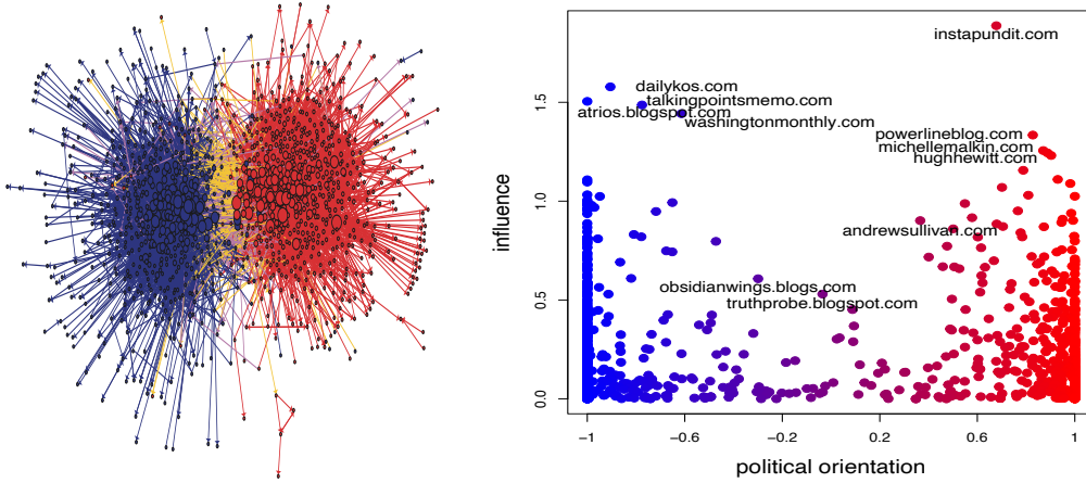
Figure 1: The political blog network and the output of Mixed-SCORE. Left: A visualization of the network (figure source: Adamic and Glance (2005) ), where blue/red colors indicate the manually assigned community labels by Adamic and Glance (2005) , and yellow/purple colors indicate the edges between two communities. Right: The estimated p_i (x-axis) and \theta_i (y-axis) by the Mixed-SCORE algorithm.
