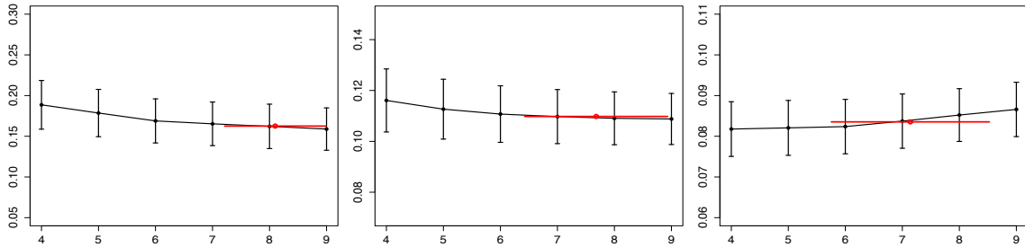
Figure 9: Performance of Mixed-SCORE as the tuning parameter L varies ( y -axis: estimation errors; \hat{L}_n^*(A) is plotted in red; both mean and standard deviation are displayed). From left to right, there are 60, 80, 100 pure nodes in each community, respectively.
